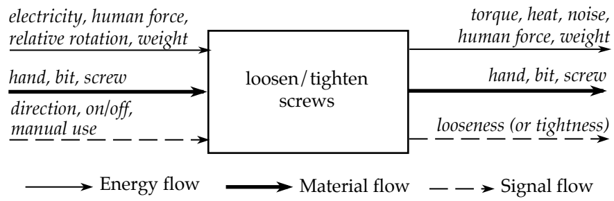
Figure 2 A Black Box model for a power screwdriver.
