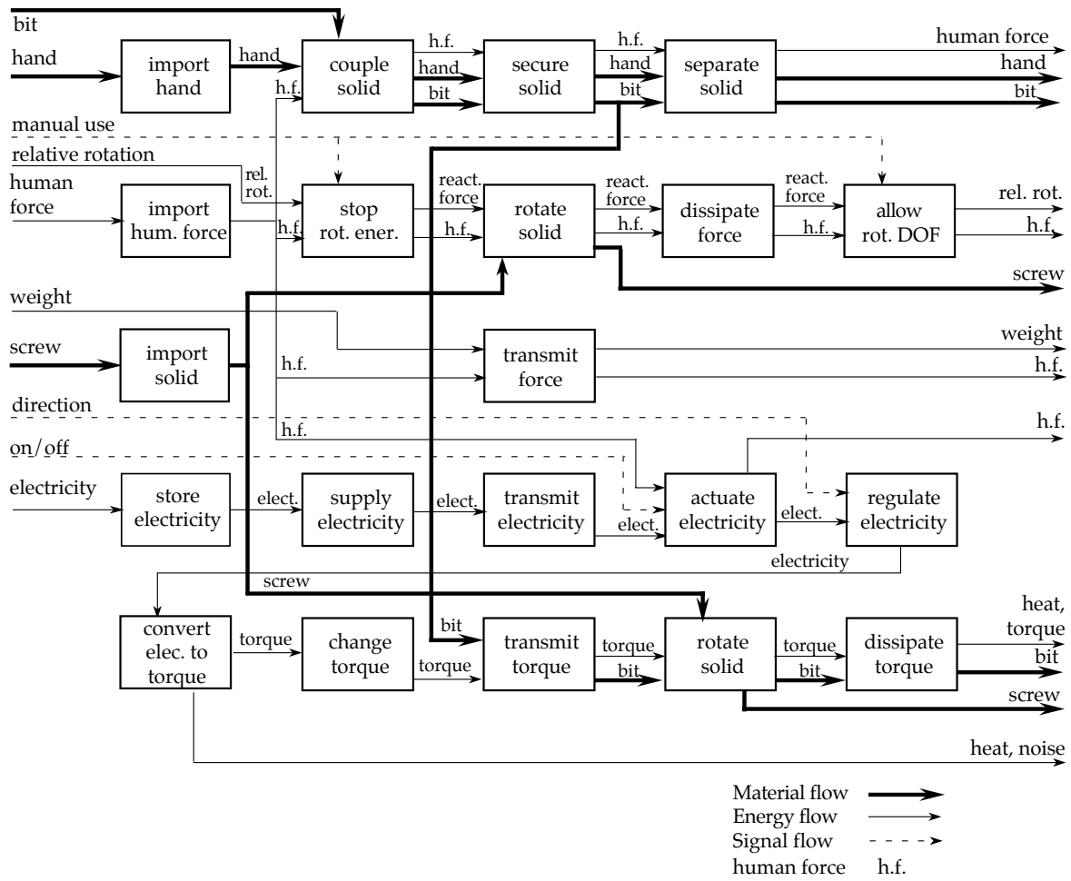
Figure 4 The functional model for a power screwdriver.
